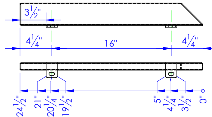
SUB-SIDERAIL 3199 RH SIDE RAIL 3200 RIGHT HAND
