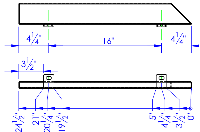
SUB-SIDERAIL 3199 RH SIDE RAIL 3200 RIGHT HAND
